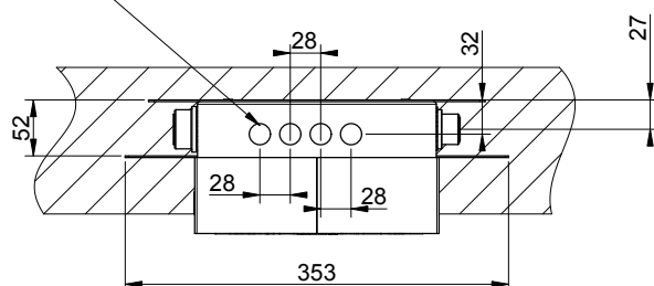
4XØ16 ELECTRICAL INLET
