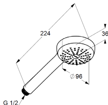
Dimensional drawing
